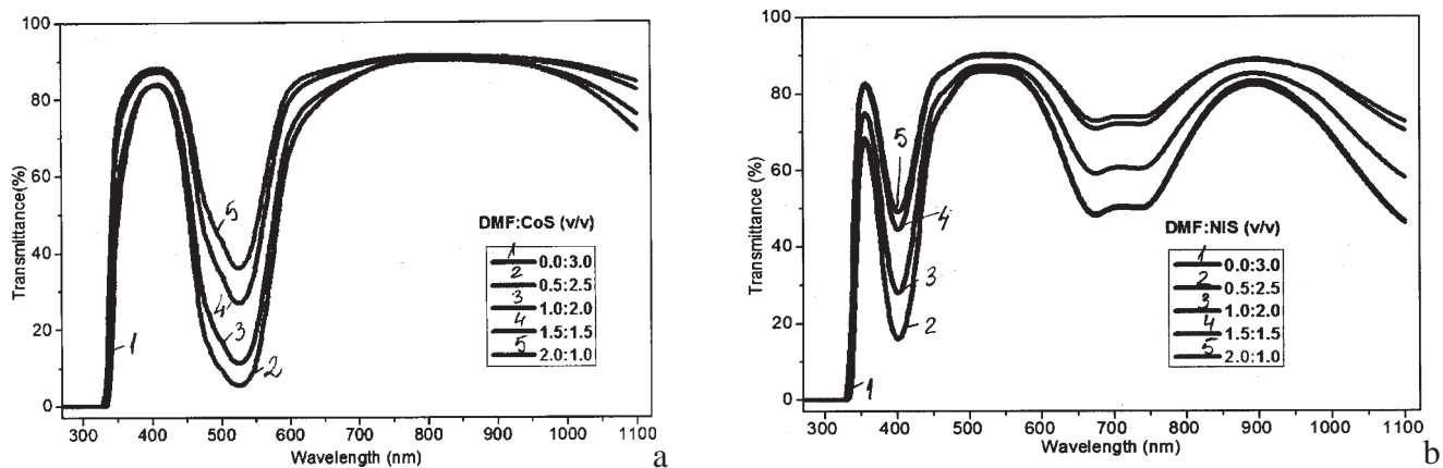
Fig. 12. The plots of the transmittance vs. wavelength of the (a) Co(II) and (b) Ni(II) complexes of the ligand for 0.0/3.0, 0.5/2.5, 1.0/2.0, 1.5/1.5 and 2.0 mL/1.0 mL DMF/Co(II) and Ni (II) solutions (v/v)
